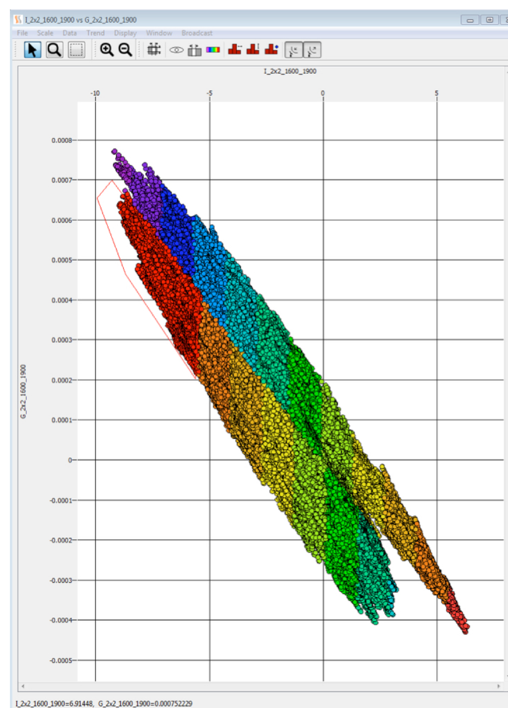
Left — Porosity Factor in color on AVO Gradient vs Intercept Xplot. Points from red polygon, projected onto AVO Gradient timeslice on Right. Possible stratigraphic trap.
