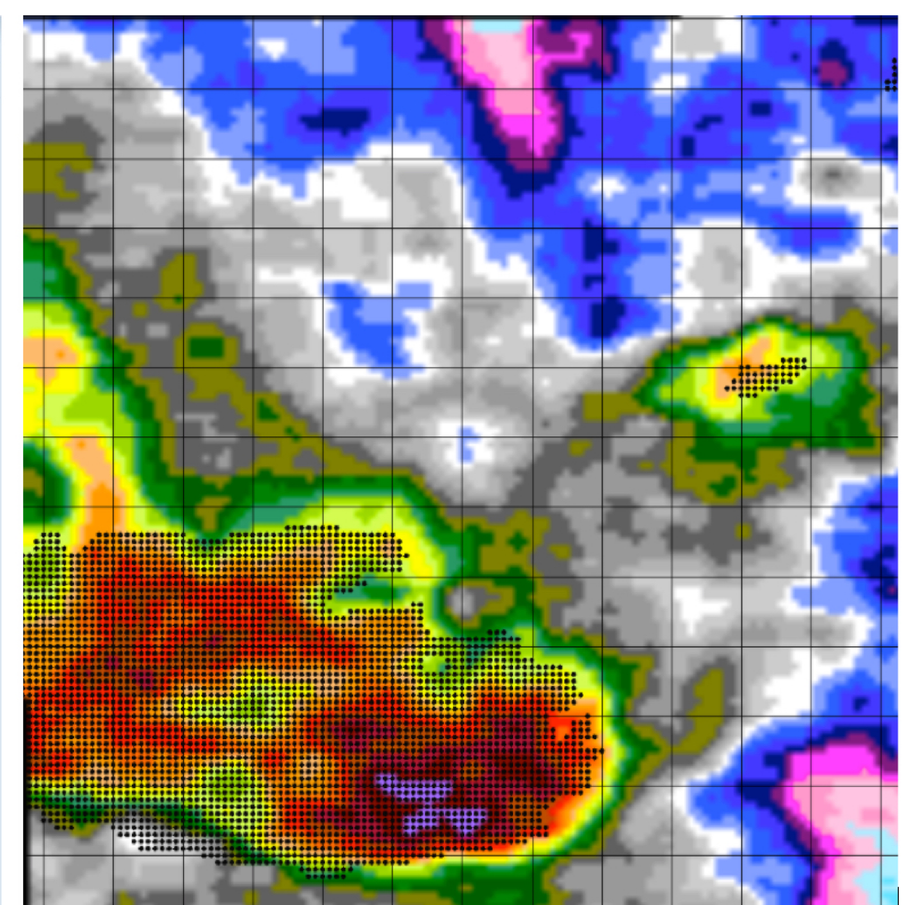
Left — Porosity Factor in color on AVO Gradient vs Intercept Xplot. Points from red polygon, projected onto AVO Gradient timeslice on Right. Possible stratigraphic trap.
